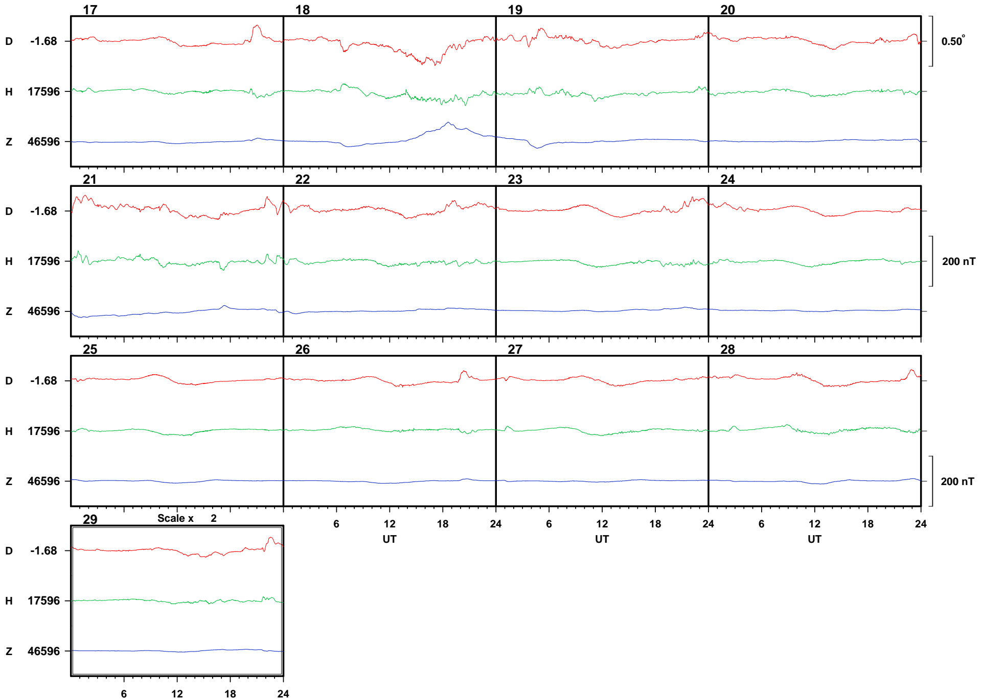
Eskdalemuir February 2020
