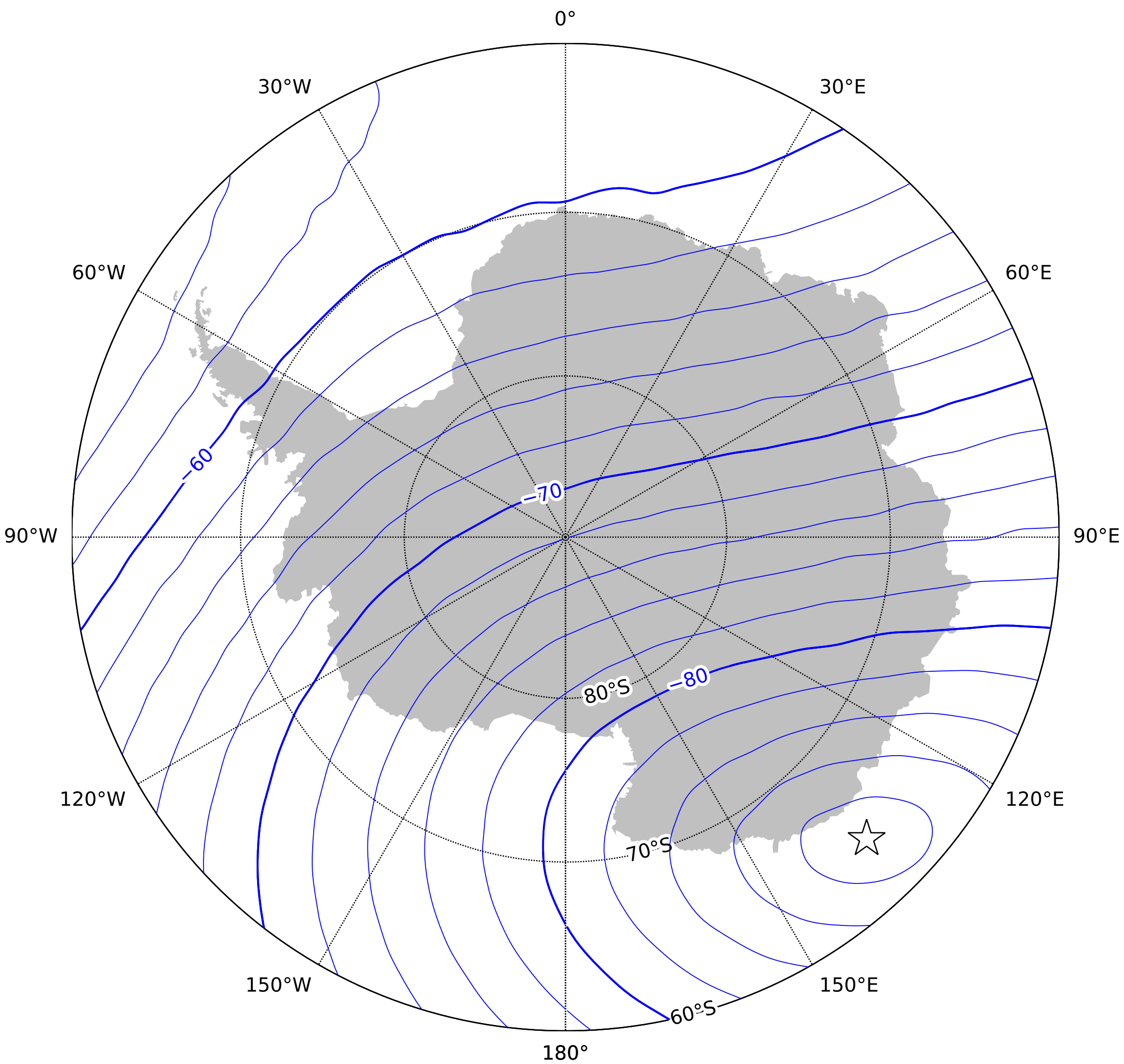
Inclination (magnetic dip) in the region of the south pole at 2025.0 from the World Magnetic Model - High Resolution (WMMHR) 2025. Red - positive (down), blue - negative (up), green - zero (dip equator). Contour interval is 2°, white star is the location of a magnetic pole and the projection is Polar Stereographic. This is an example of an isoclinic chart.
