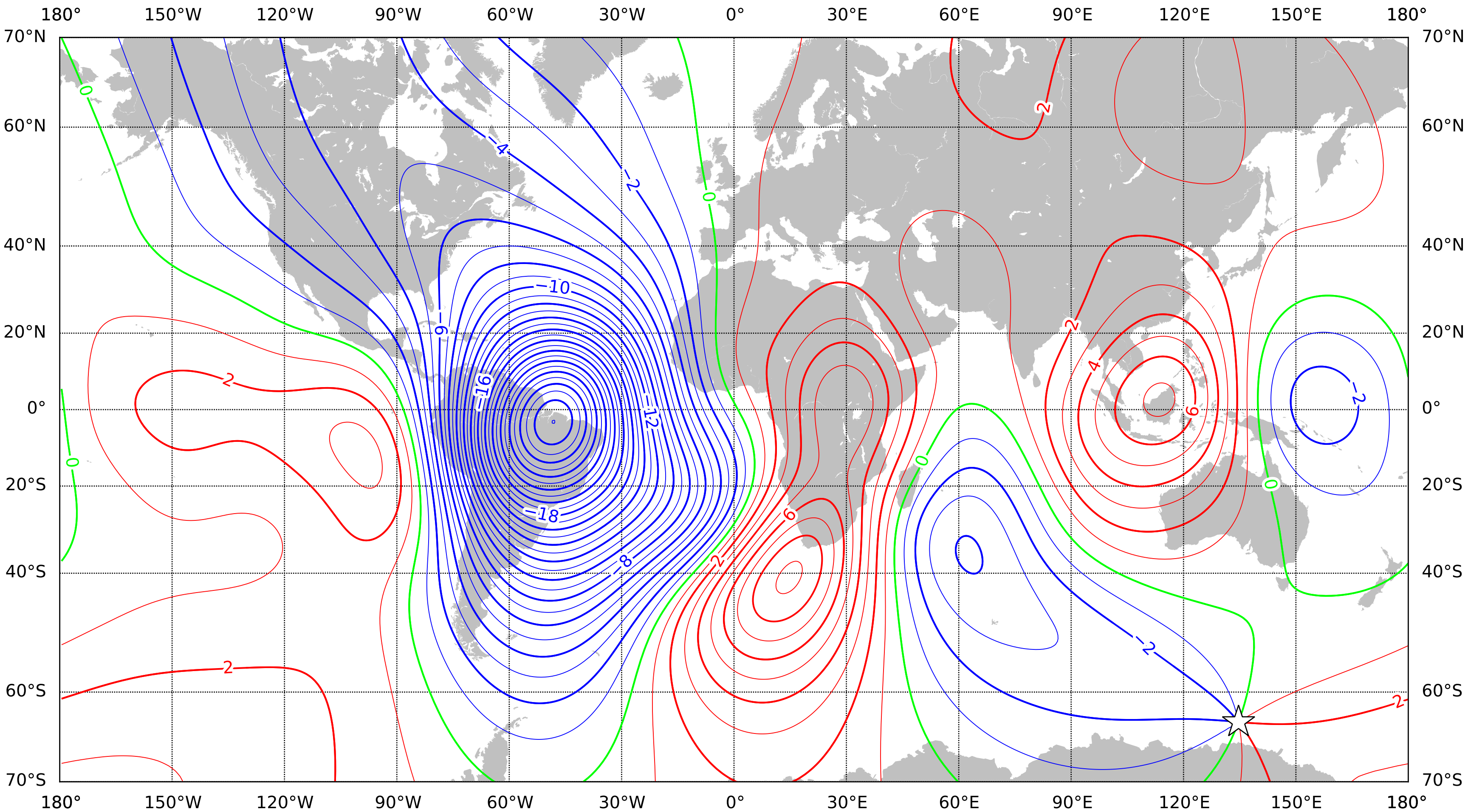
Annual rate of change of inclination at 2027.5 from the World Magnetic Model - High Resolution (WMMHR) 2025 (core component only). Red - positive (downward) change, blue - negative (upward) change, green - zero change. Contour interval is 1/year, white star is the location of a magnetic pole and the projection is Mercator. This is an example of an isoporic chart.
