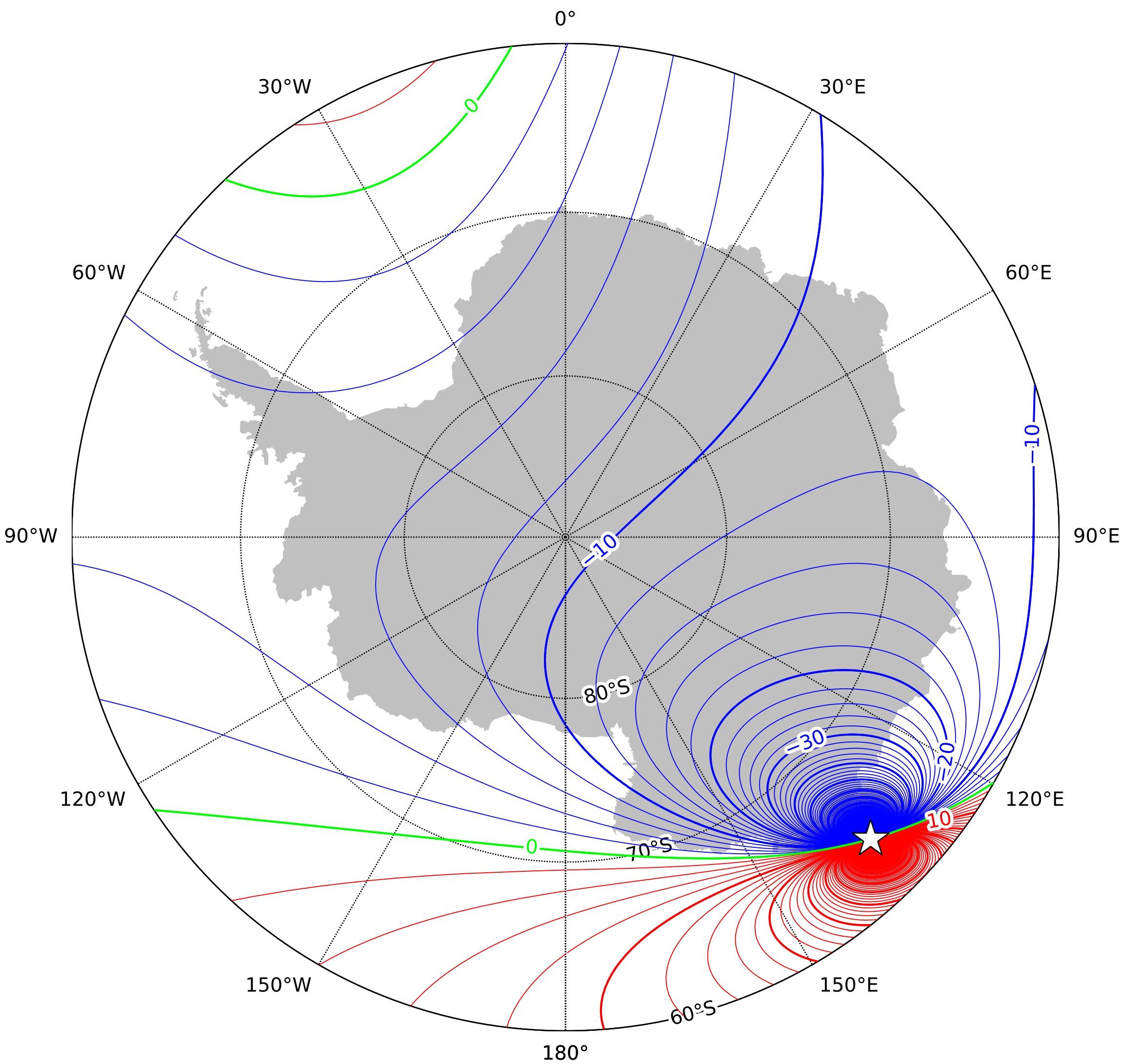
Annual rate of change of declination in the region of the south pole at 2027.5 from the World Magnetic Model - High Resolution (WMMHR) 2025 (core component only). Red - positive (easterly) change, blue - negative (westerly) change, green - zero change. Contour interval is 2'/year, white star is the location of a magnetic pole and the projection is Polar Stereographic. This is an example of an isoporic chart. British Geological Survey © UKRI 2024
