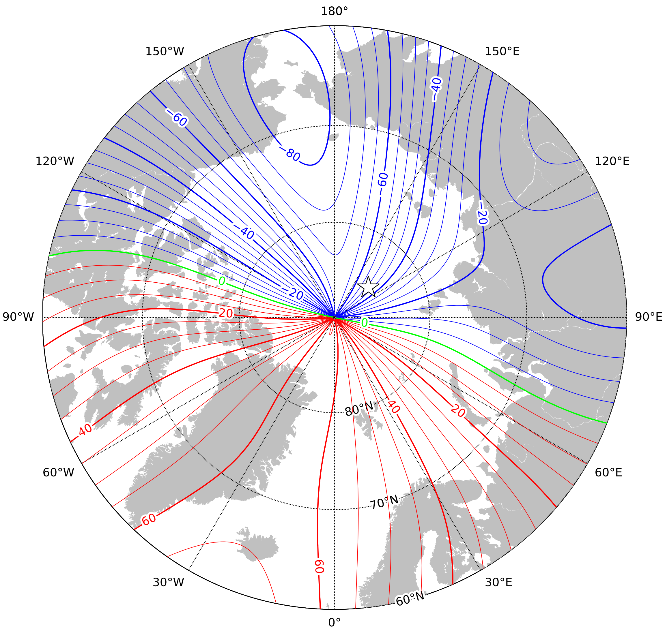
Annual rate of change of east component in the region of the north pole at 2027.5 from the World Magnetic Model (WMM) 2025. Red - positive (easterly) change, blue - negative (westerly) change, green - zero change. Contour interval is 5nT/year, white star is the location of a magnetic pole and the projection is Polar Stereographic. This is an example of an isoporic chart. British Geological Survey © UKRI 2024
