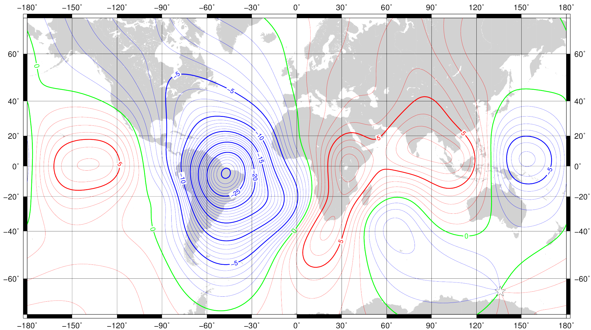
Annual rate of change of inclination for 2020.0 to 2025.0 from the World Magnetic Model (WMM2020). Red – positive (down) change, blue – negative (up) change, green – zero change. Contour interval is 1°/year, white star is location of a magnetic pole and projection is Mercator. This is an example of an isoporic chart. Credit: British Geological Survey (UK Research and Innovation).
