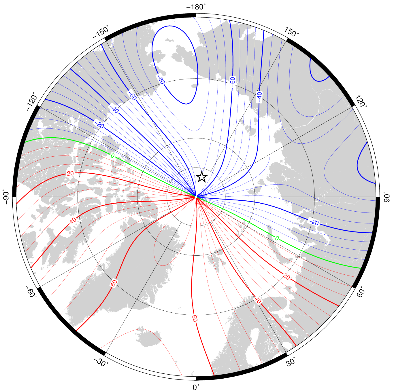
Annual rate of change of east component in region of north pole for 2020.0 to 2025.0 from the World Magnetic Model (WMM2020). Red – positive change, blue – negative change, green – zero change. Contour interval is 5 nT/year, white star is location of a magnetic pole and projection is Polar Stereographic. Credit: British Geological Survey (UK Research and Innovation).
