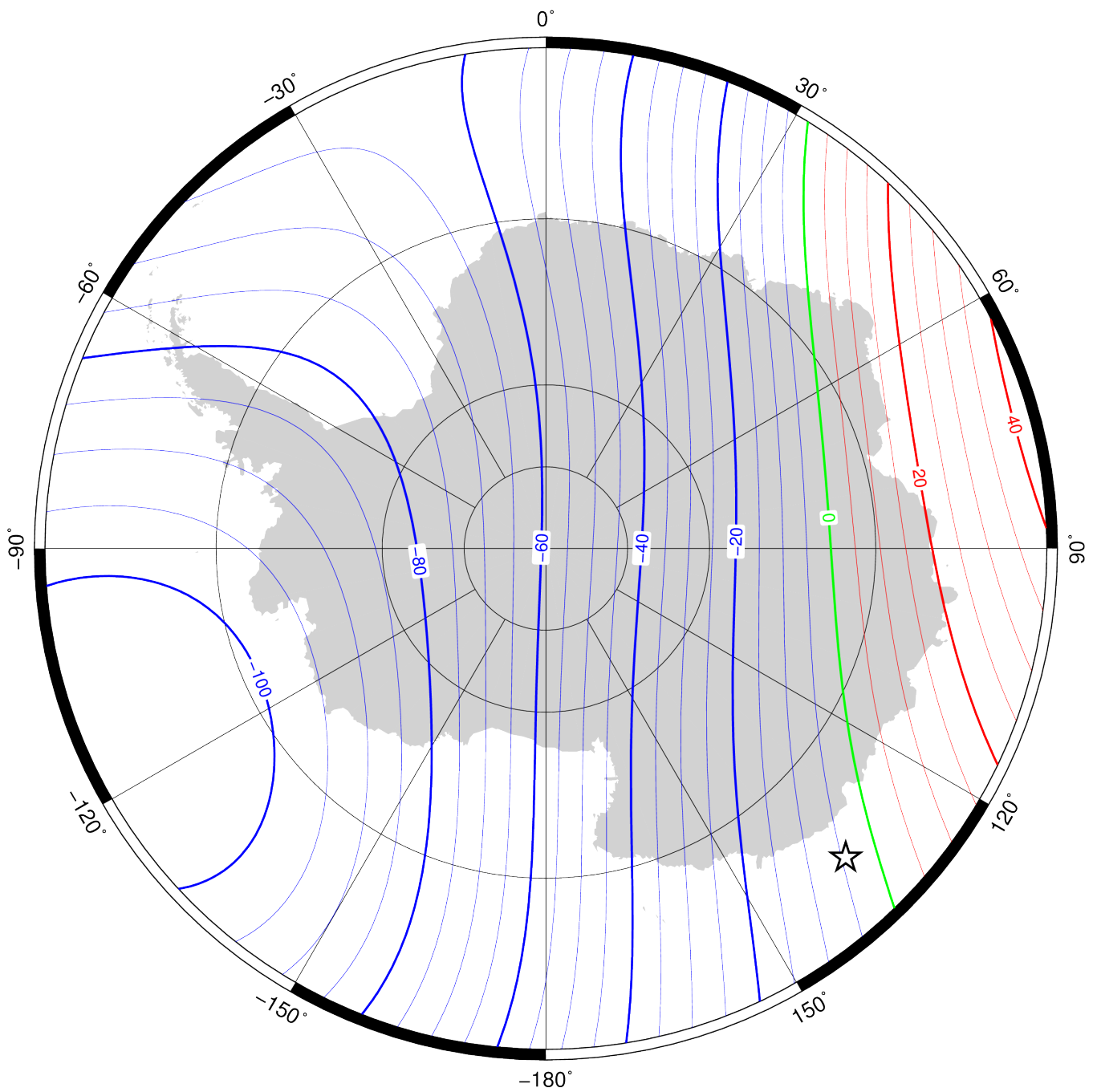
Annual rate of change of total intensity in region of south pole for 2020.0 to 2025.0 from the World Magnetic Model (WMM2020). Red – positive change, blue – negative change, green – zero change. Contour interval is 5 nT/year, white star is location of a magnetic pole and projection is Polar Stereographic. Credit: British Geological Survey (UK Research and Innovation).
