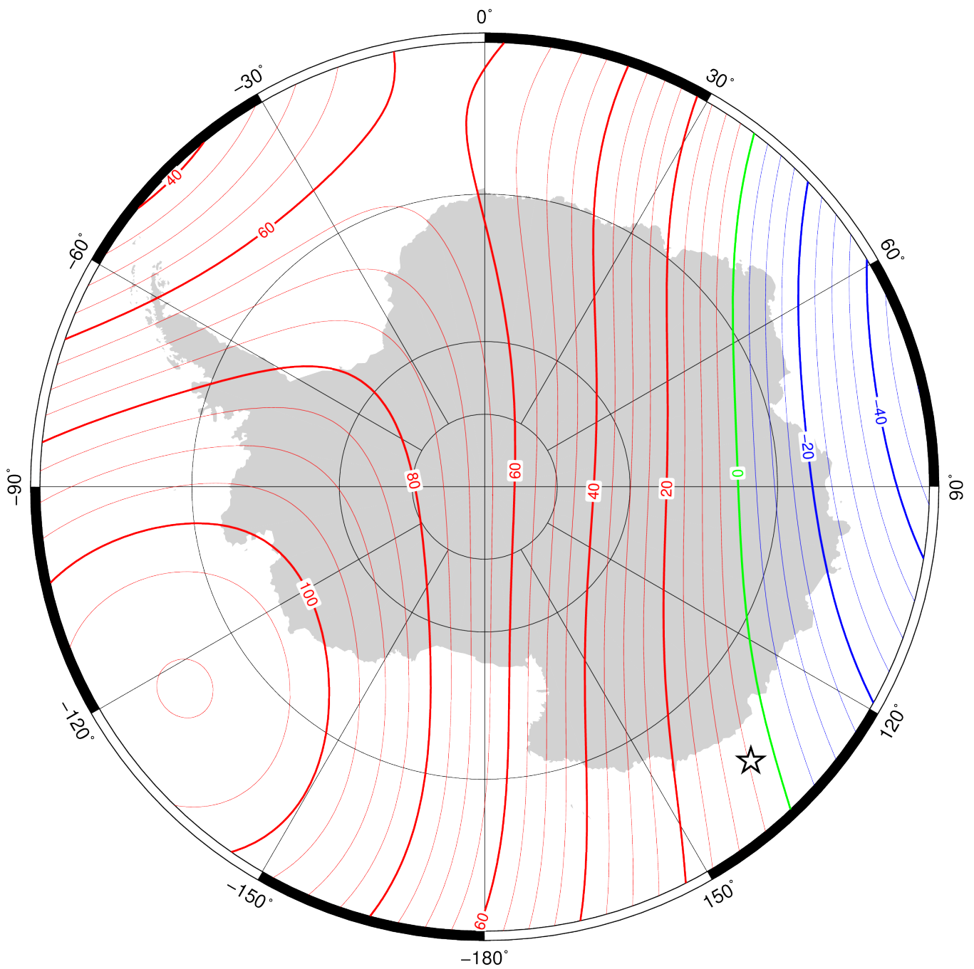
Annual rate of change of vertical component in region of south pole for 2020.0 to 2025.0 from the World Magnetic Model (WMM2020). Red – positive change, blue – negative change, green – zero change. Contour interval is 5 nT/year, white star is location of a magnetic pole and projection is Polar Stereographic. Credit: British Geological Survey (UK Research and Innovation).
