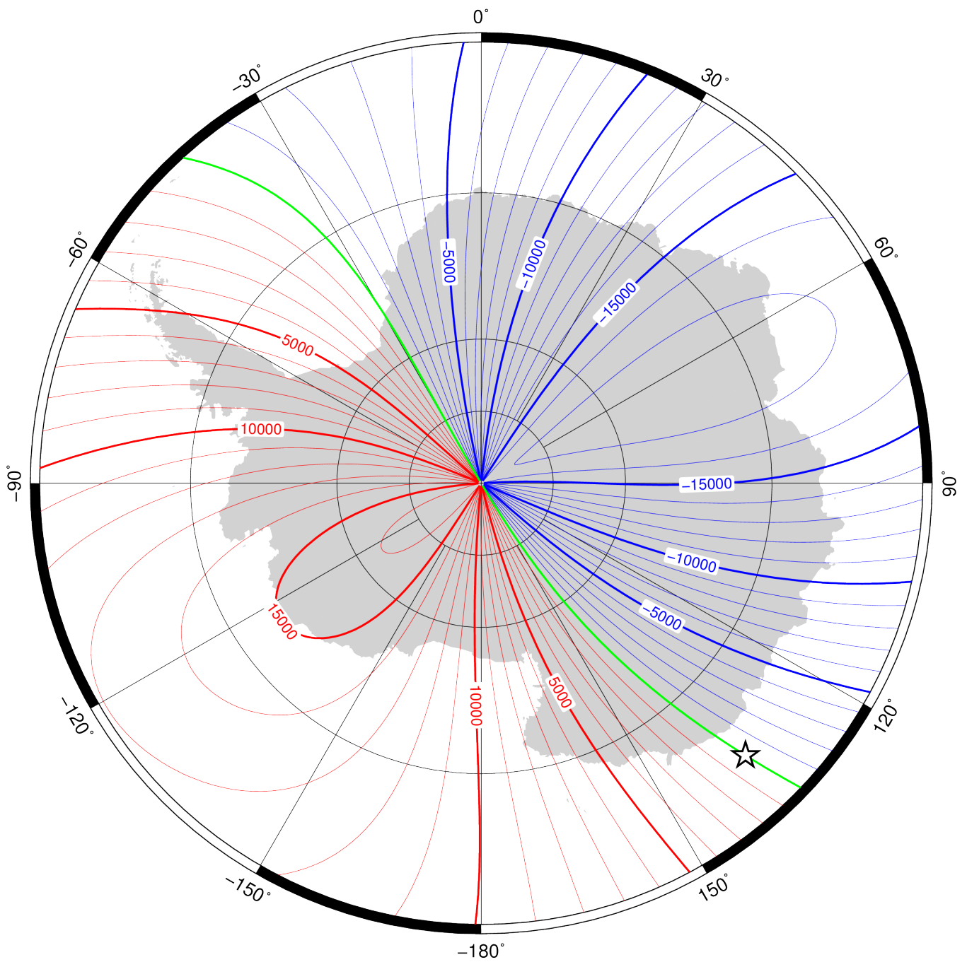
East component ( Y ) in region of south pole at 2020.0 from the World Magnetic Model (WMM2020). Red – positive (east), blue – negative (west), green – zero. Contour interval is 1000 nT, white star is location of a magnetic pole and projection is Polar Stereographic. Credit: British Geological Survey (UK Research and Innovation).
